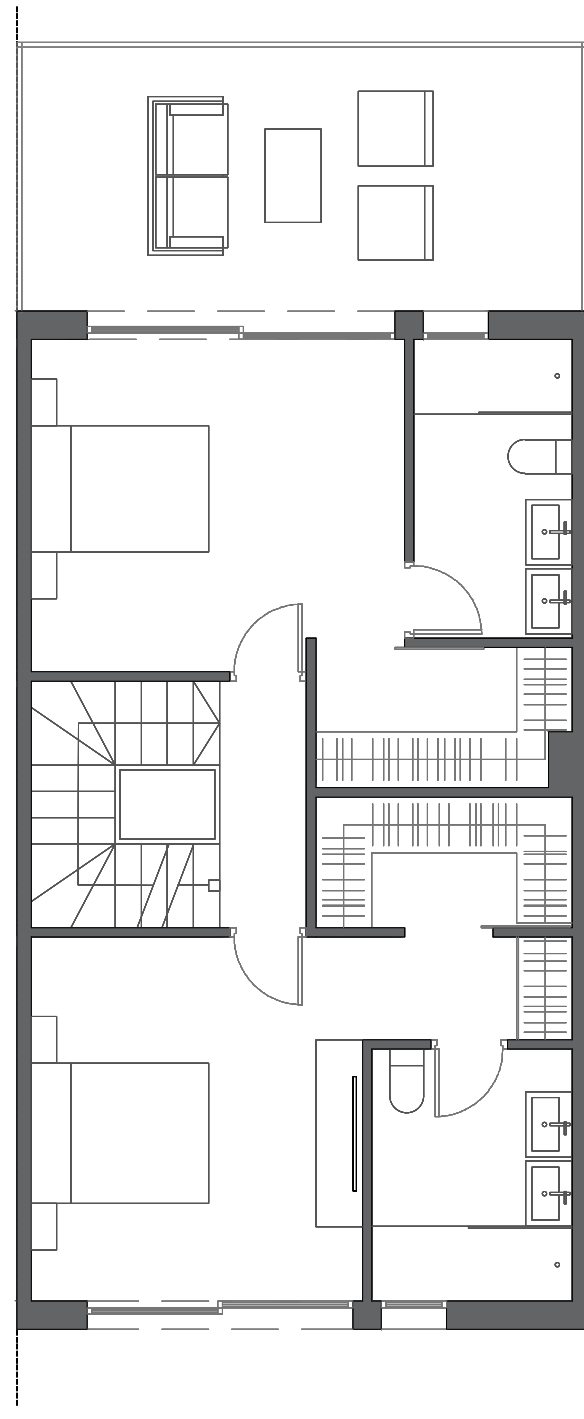
FIRST FLOOR - C
